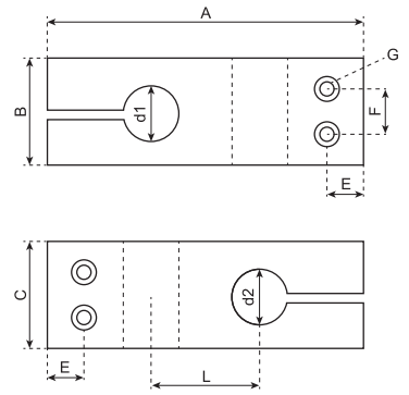
N200B 系列同径双孔十字夹 (双螺栓型) N200B SAME DIAMETER DOUBLE HOLE CROSS CLAMP (DOUBLE BOLT)
