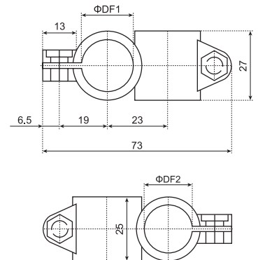
N202T 十字承夹 N202T CROSS CLAMP
