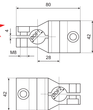
N202SS-2 十字承夹 N202SS-2 CROSS CLAMP
