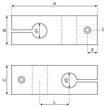
N200A 系列同径双孔十字夹 (单螺栓型) N200A SAME DIAMETER DOUBLE HOLE CROSS CLAMP (SINGLE BOLT)
