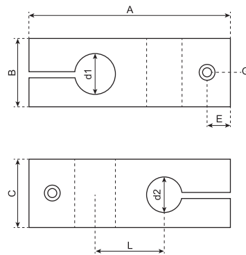
N200C 系列异径双孔十字夹 (单螺栓型) N200C UNEQUAL DIAMETER DOUBLE HOLE CROSS CLAMP (SINGLE BOLT)
