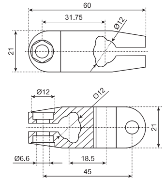
N201SS 十字承夹 N201SS CROSS CLAMP
